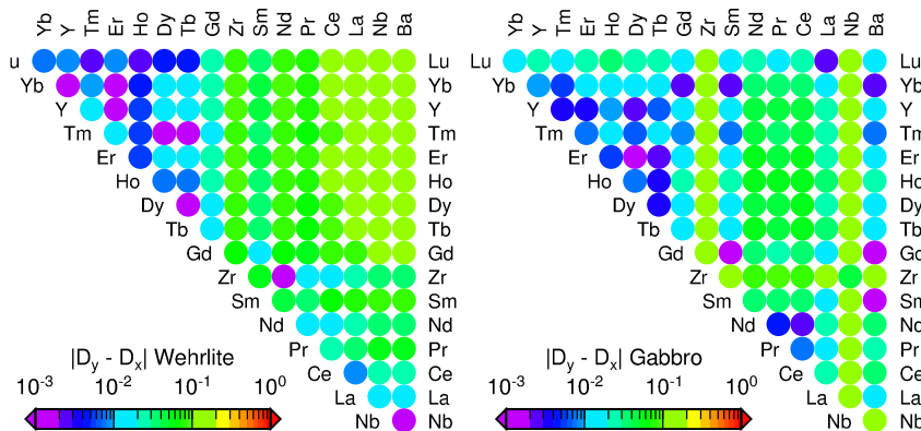
Fig. B.4. The absolute difference in bulk partition coefficients if olivine, plagioclase and clinopyroxene are crystallising in wehrlitic the proportions (ol 69 plag 1 cpx 30 ) or gabbroic (ol 7 plag 53 cpx 40 ) proportions.
