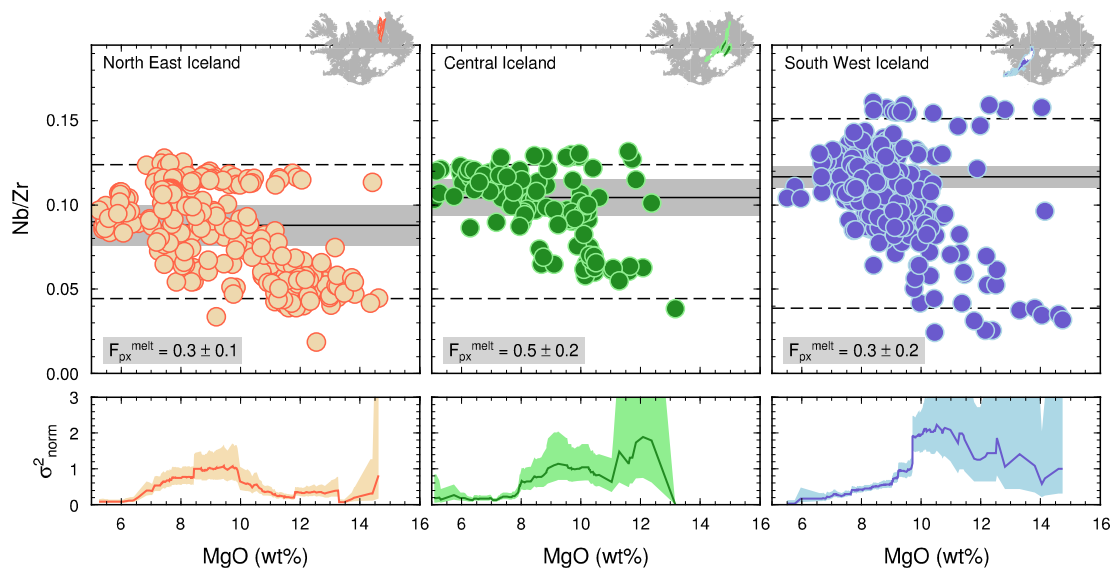
Fig. 1. The geochemical variability recorded in Icelandic whole-rock samples. The top three panels show how in lavas from each zone Nb/Zr evolves as MgO drops. Solid horizontal lines mark the volume average composition (Nb/Zr) calculated from all samples in the zone, with 1 s.e. drawn as a grey bar (see text for details). Dashed horizontal lines record the endmember Nb/Zr calculated from the highest and lowest 10% of samples from each zonal dataset (5% for south west Iceland, because of its smaller number of samples at enriched and depleted extremes) falling within a 9.5–12 wt% MgO interval (Shorttle and MacLennan, 2011). F_{px}^{melt} is calculated using Eq. (4), which mass balances the endmember compositions with the volume average crustal composition shown in each panel, uncertainty on F_{px}^{melt} is propagated from the standard deviation of the endmember compositions and mean crustal composition and quoted at 1\sigma . Inset maps highlight the geographic location of each volcanic system the samples are from. The bottom panels show the running normalised variance for the data in the plots above, binned in 1.5 wt% MgO intervals with a 95% confidence envelope. Data sources can be found in Appendix F.
