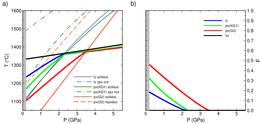
Fig. D.6. Results of model calculations melting single lithology mantles of Iherzolite (lz), pyroxenite (G2 or KG1, Pertermann and Hirschmann, 2003 ; Kogiso et al., 1998 ) or harzburgite (hz) at a mantle potential temperature of 1330 °C. (a) Pressure–temperature paths for a column of single lithology mantle undergoing isentropic decompression, followed by melting once it has intersected its solidus. Mantle P – T paths are indicated by thick solid lines, solidus, liquidus and clinopyroxene out (cpx out) boundaries for each lithology are marked by thin solid or dashed lines. Because the harzburgite is constrained to undergo no melting it defines a simple adiabat (Eq. (D.3)) for the whole pressure range. The shaded area marks the crustal thickness applied in these calculations, and therefore the pressure at which the melting calculations stop. (b) The degree of melting for a packet of mantle undergoing the maximum amount of decompression.
